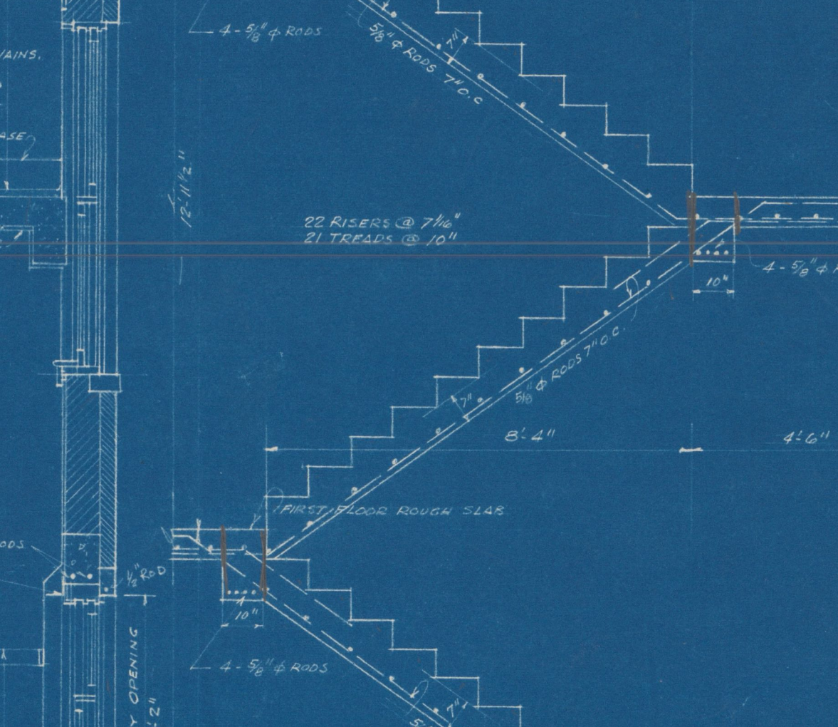
SECTION 'A'-A' SHOWING STRUCTURAL CONCRETE STEPS AND LANDINGS SCALE 3/8"=1'-0"
