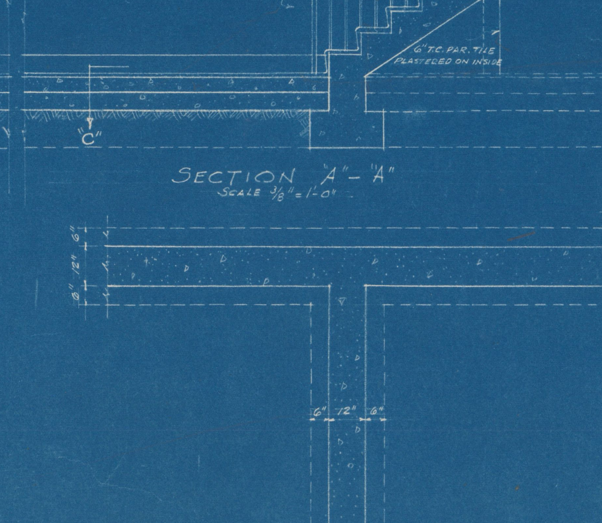
TYPICAL REAR STAIRS
