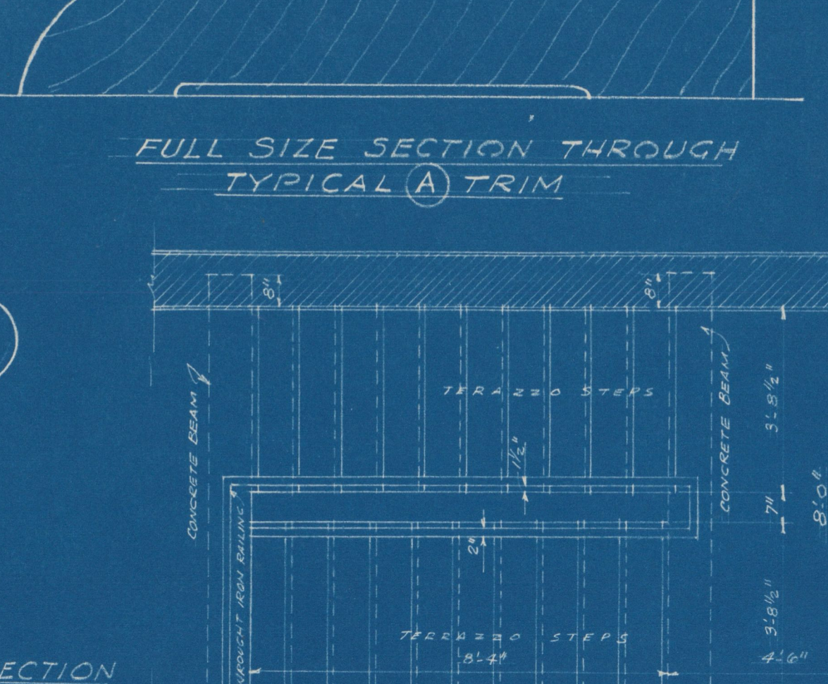
FULL SIZE SECTION THROUGH TYPICAL (A) TRIM
