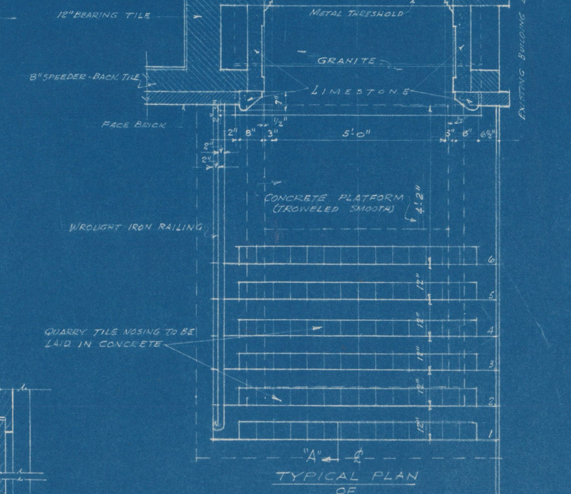
TYPICAL PLAN OF REAR PLATFORMS SCALE 3/8"=1'-0"
