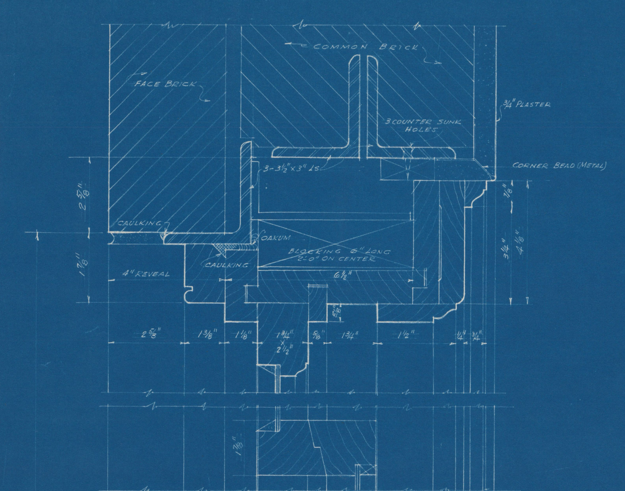
SECTION THROUGH MULLION ONE HALF FULL SIZE
