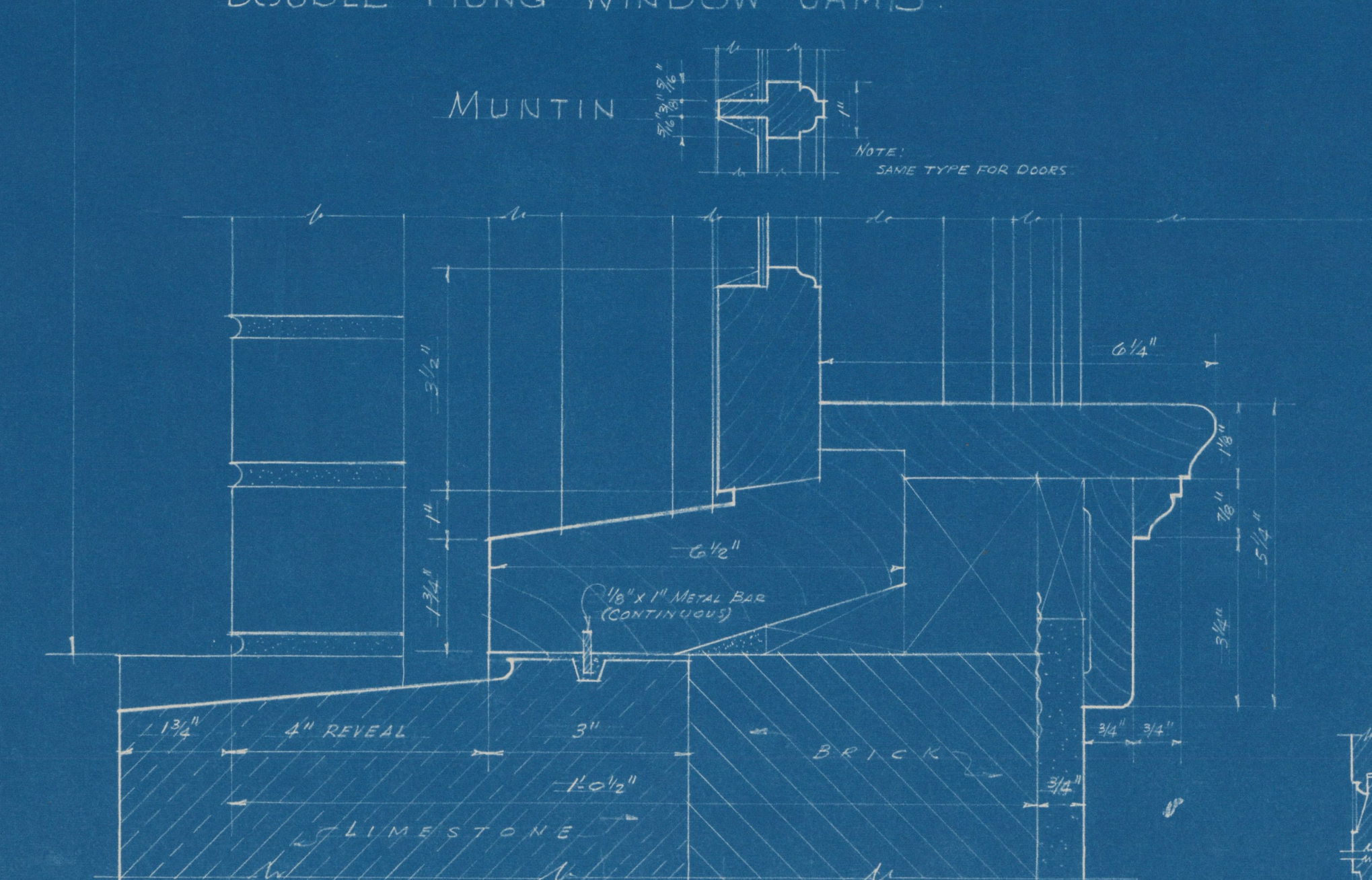
DETAILS OF DOUBLE HUNG WINDOW ONE HALF FULL SIZE
