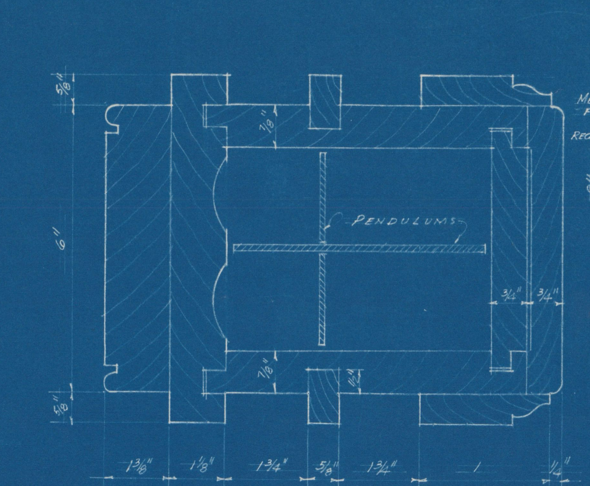
SECTION THROUGH MULLION ONE HALF FULL SIZE
