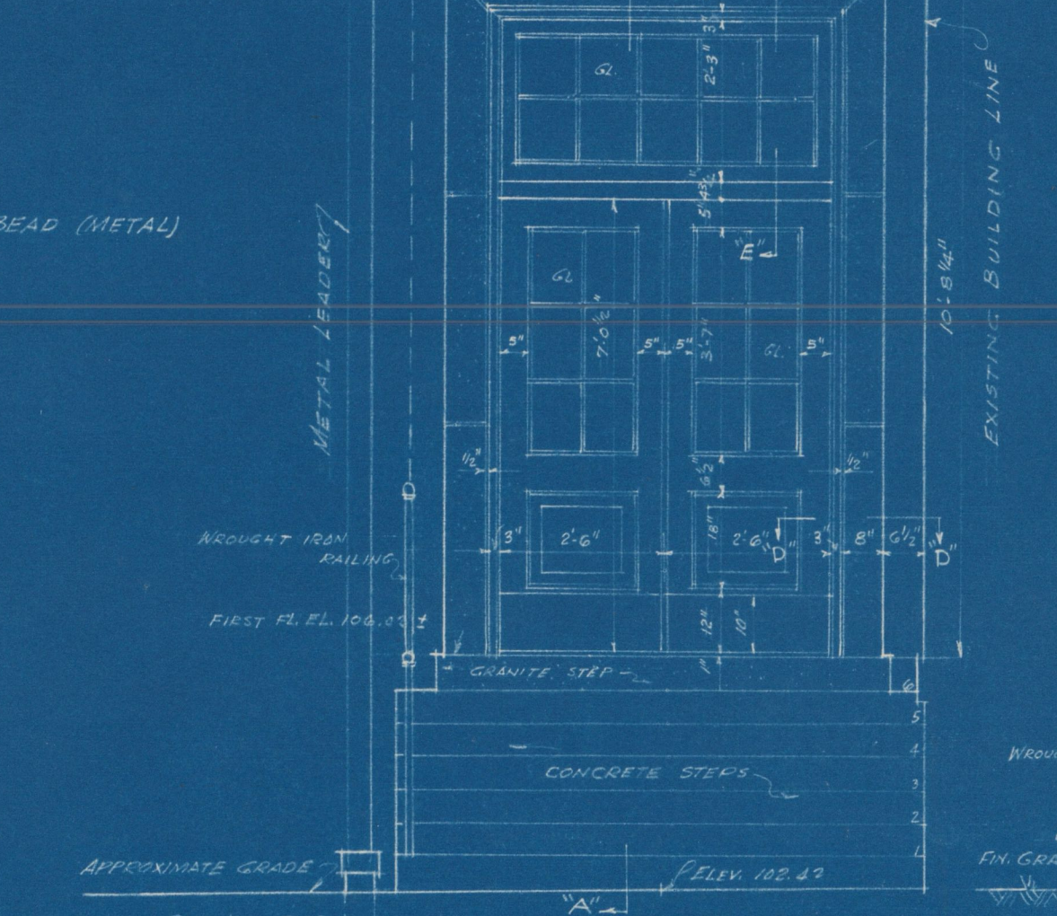
TYPICAL ELEVATION OF REAR DOORS SCALE 3/8"=1'-0"
