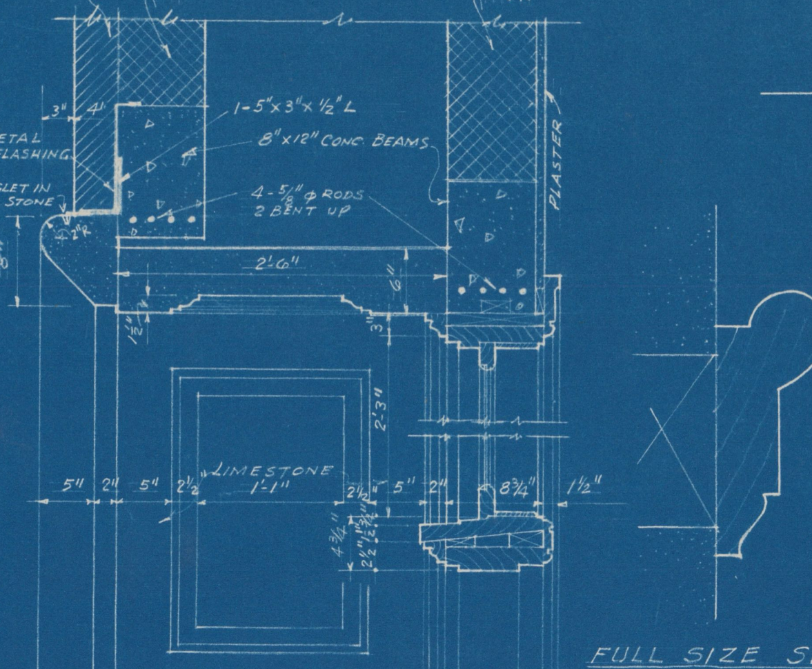
SECTION 'E'-E' TYPICAL REAR DOORS SCALE 1/2"=1'-0"
